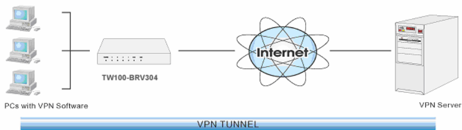
Figure 45: VPN Pass-through
