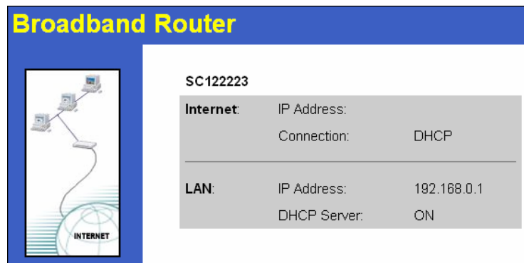
Figure 6: Home Screen
