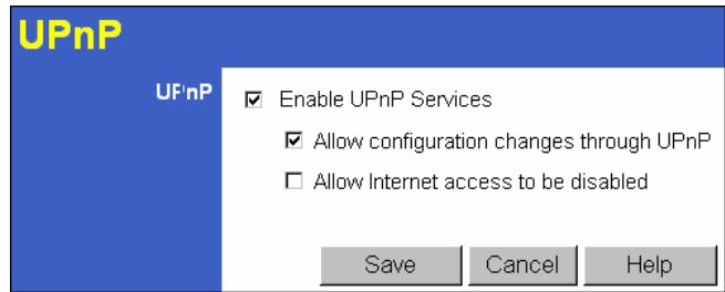
Figure 119: UPnP Screen
