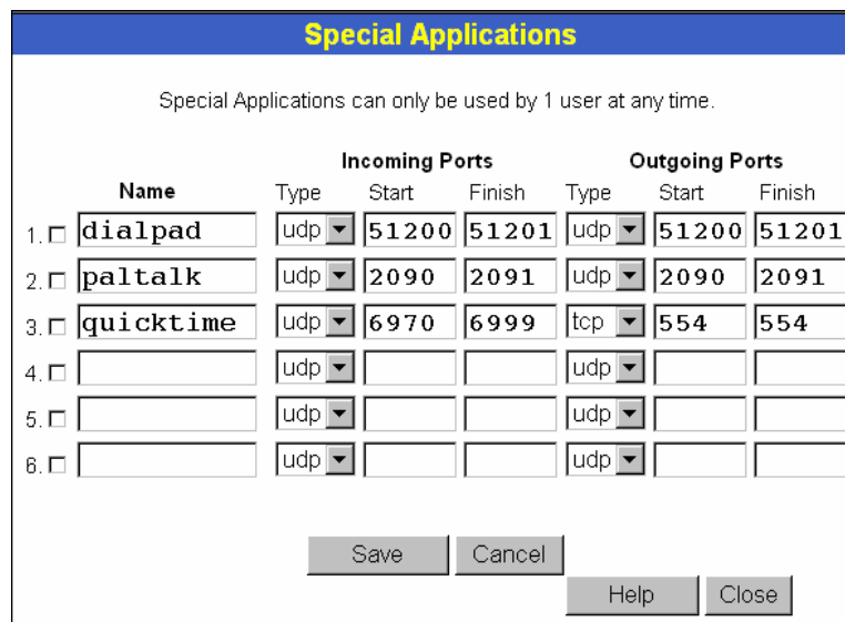
Figure 28: Special Applications Screen
