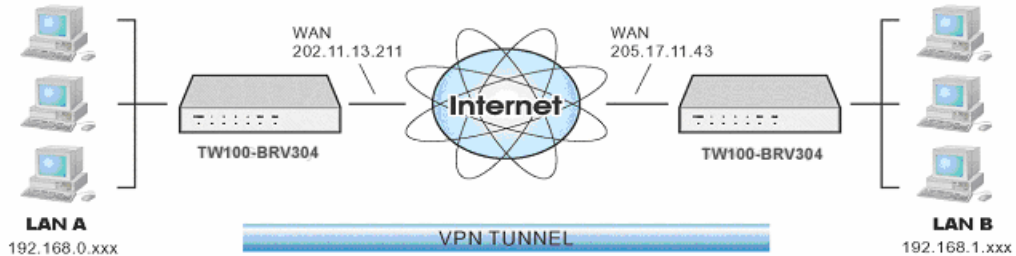
Figure 56: Connecting 2 TW100-BRV304s
