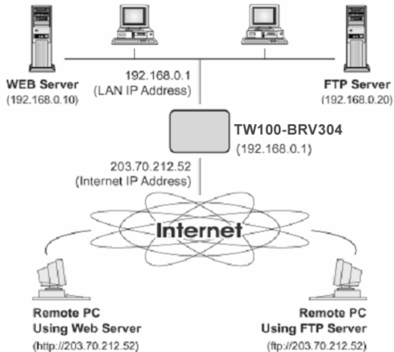
Figure 31: Virtual Servers
