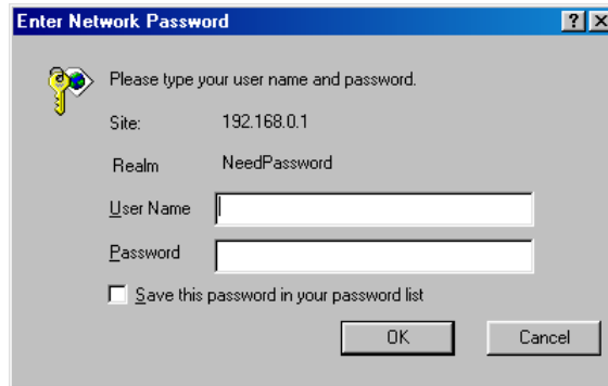
Figure 35: Password Dialog
