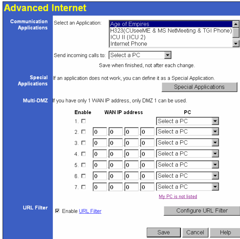
Figure 27: Internet Screen
