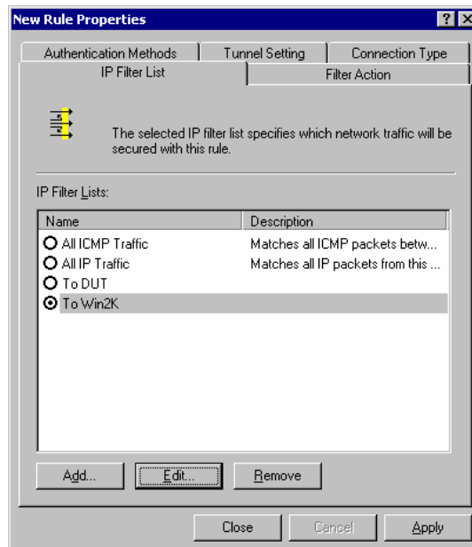
Figure 72: Filter List
