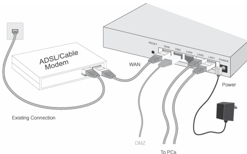
Figure 4: Installation Diagram
