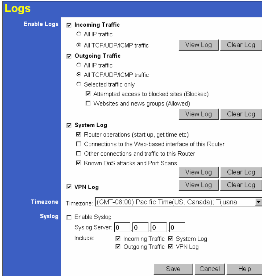
Figure 40: Logs Screen
