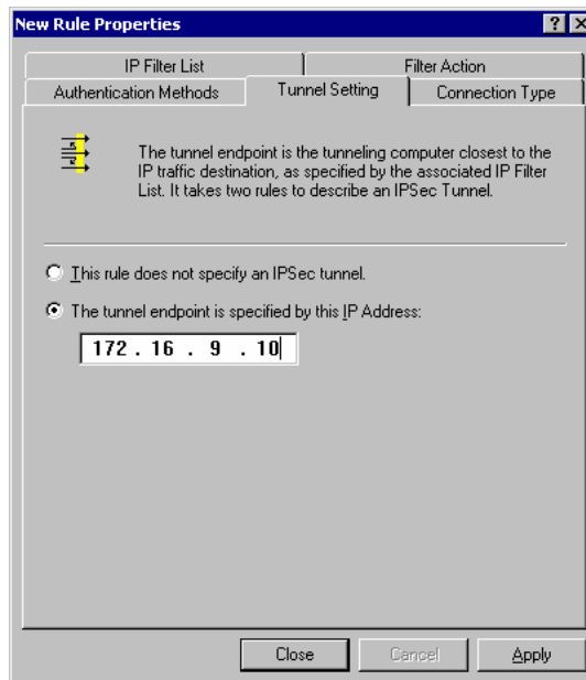
Figure 76: Tunnel Setting
