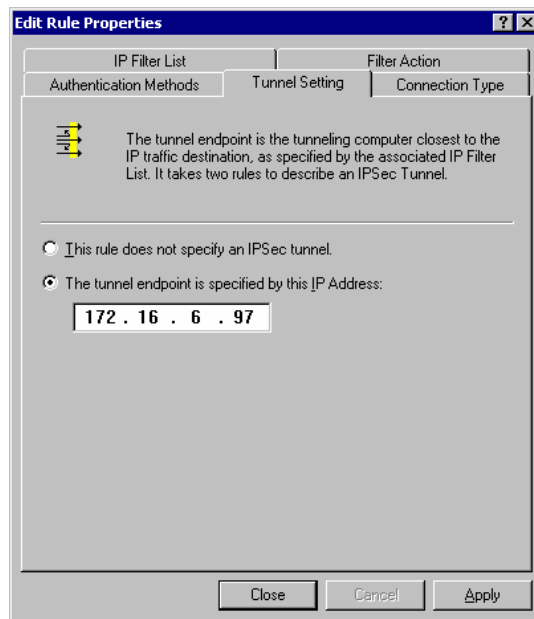
Figure 67: Tunnel Setting
