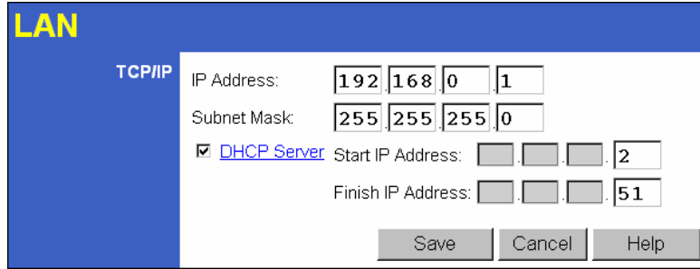
Figure 7: LAN Screen
