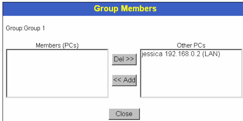
Figure 37: Group Members
