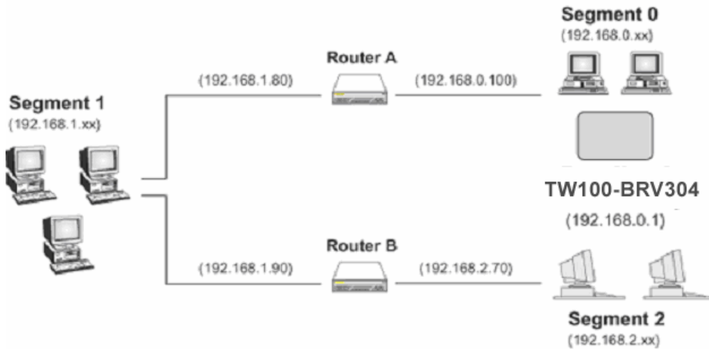
Figure 117: Routing Example
