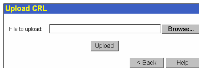
Figure 93: Upload CRL
