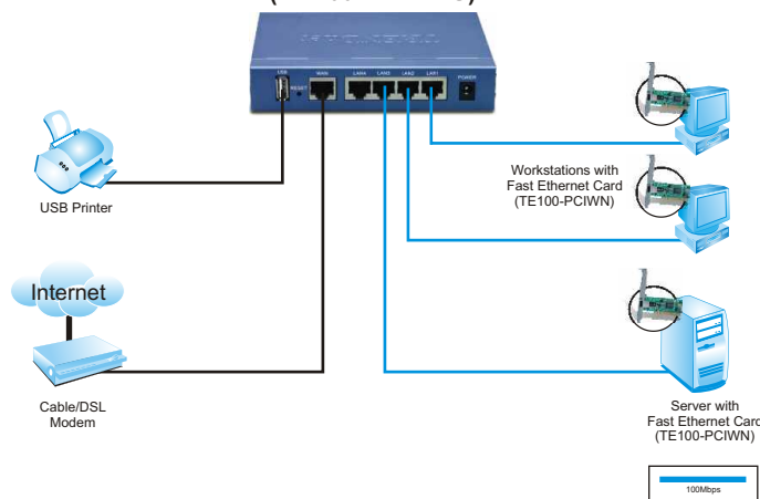
Cable/DSL 4-Port Firewall Router with USB Print Server (TW100-BRF114U)
