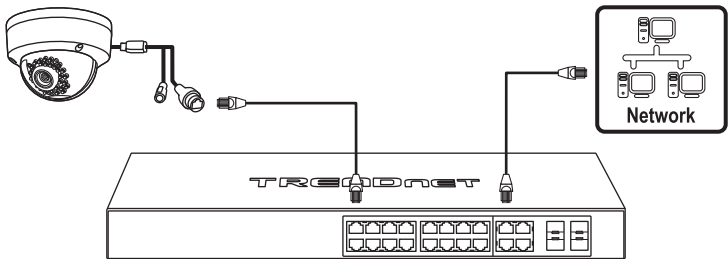
PoE Camera
