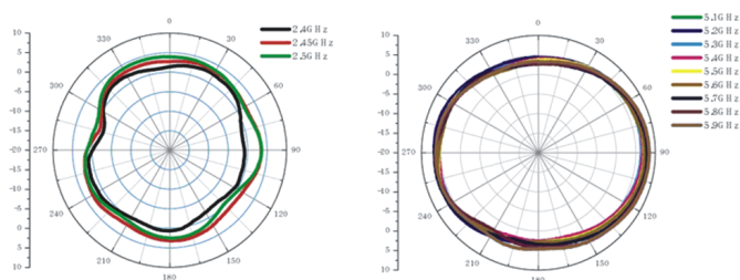
H-plane Co-polarization pattern
