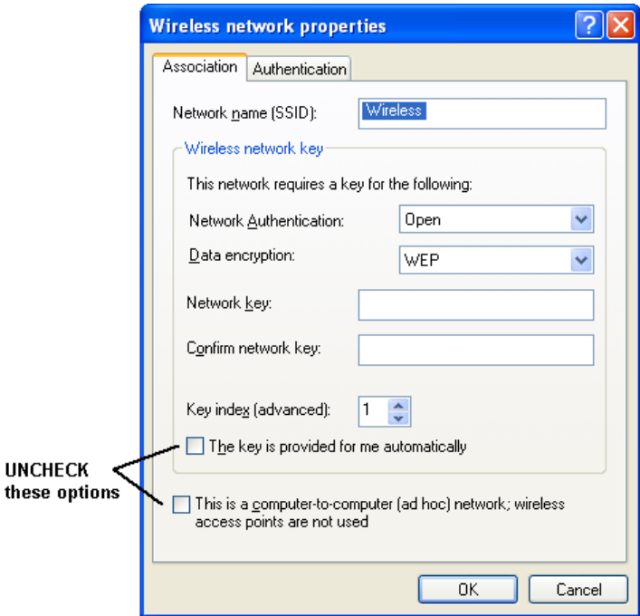
Figure 38: Wireless Network Properties - WEP
