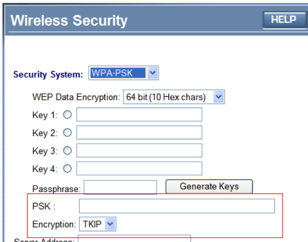
Figure 14: WPA-PSK
