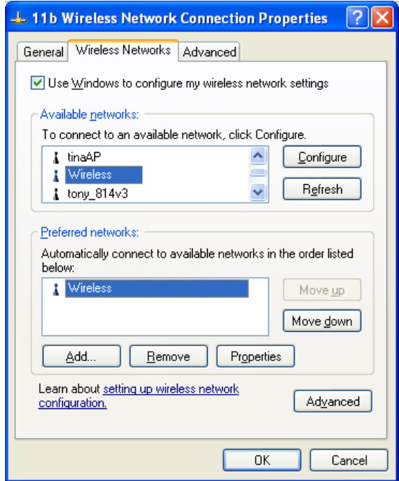
Figure 39: Preferred Networks
