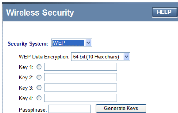
Figure 13: WEP
