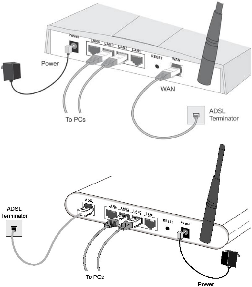
Figure 4: Installation Diagram
