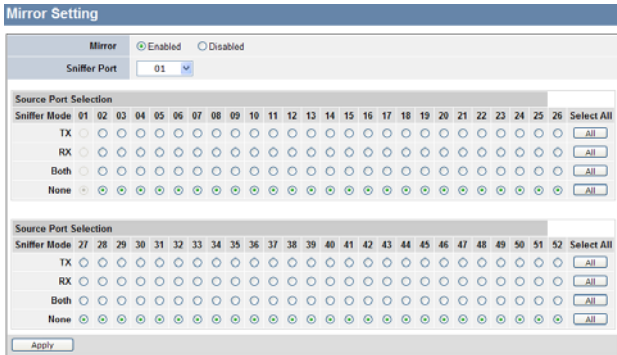
Figure 23. Mirror Setting
