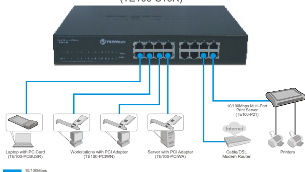
16-Port 10/100Mbps Fast Ethernet Switch (TE100-S16R)
